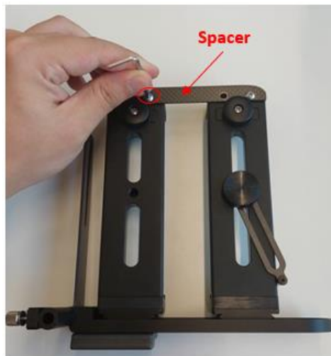
Figure 21 Loosen spacer by loosen the screws.
