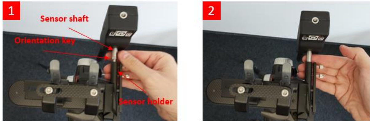
Figure 12 Mounting the sensor.
