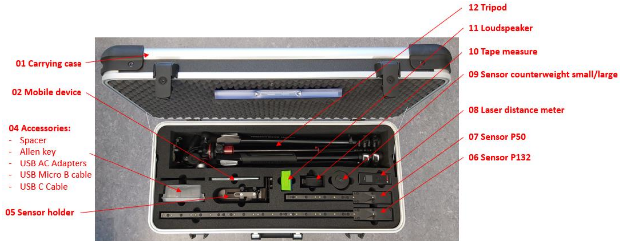
Figure 3 Content of case without hinged lid.
