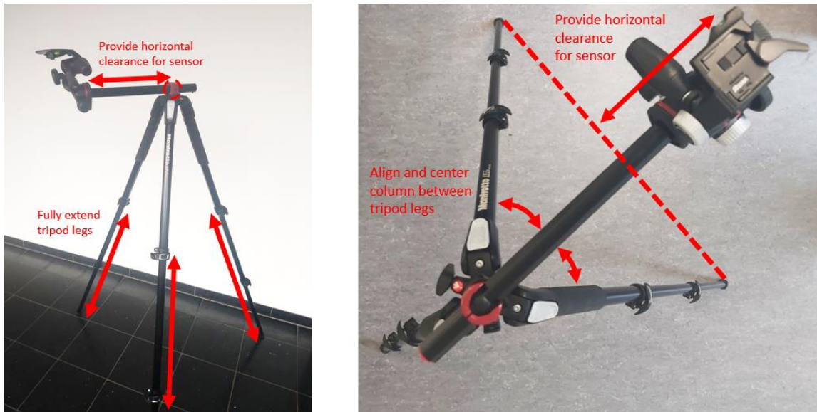
Figure 10 Fully extend tripod legs for sensor P254 and provide horizontal clearance by pulling out the extendable column (left), align extendable column between tripod legs (right).
