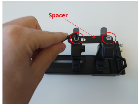
Figure 18 Loosen the screws to remove the spacer from the clamps.
