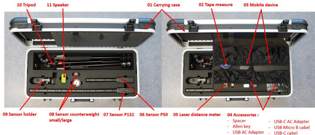
Figure 2 Content of case with hinged lid.
