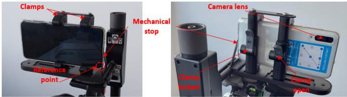
Figure 16 Insert the mobile device in the holder and check its orientation.
