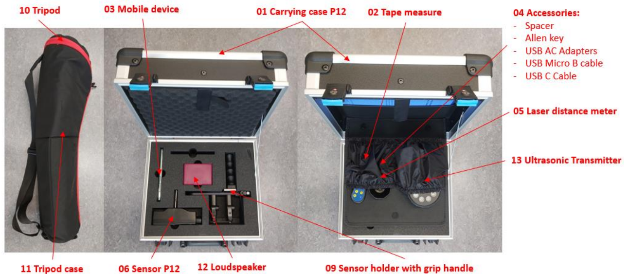
Figure 1 Content of case P12 with hinged lid
